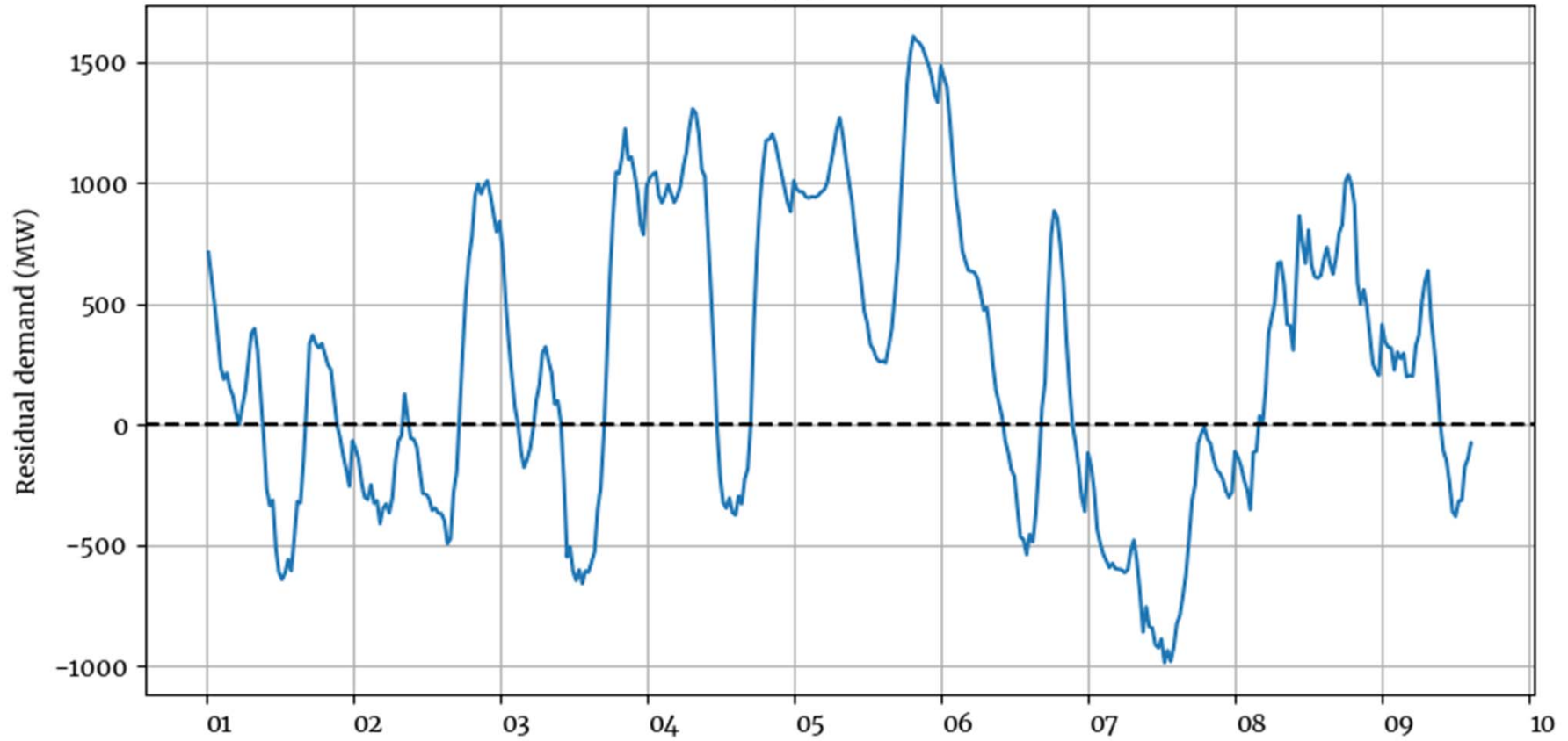
Residual demand, South Australia (Sept 2020)
