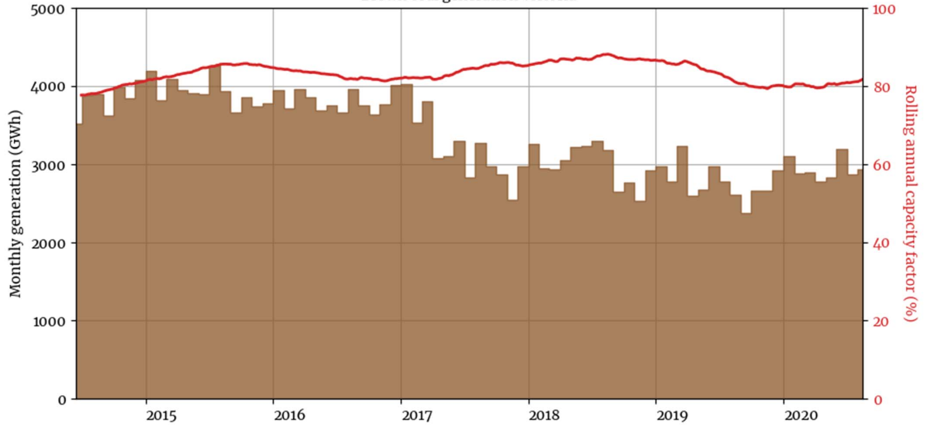
Brown coal generation Victoria
