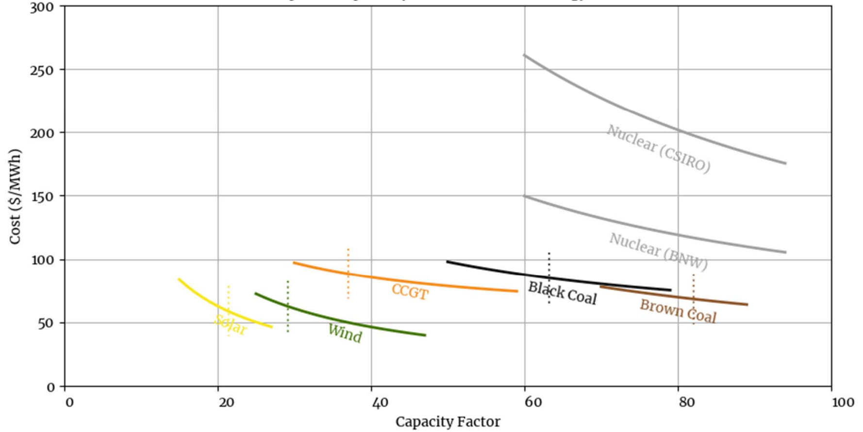
Impact of capacity factor on levelised energy costs
